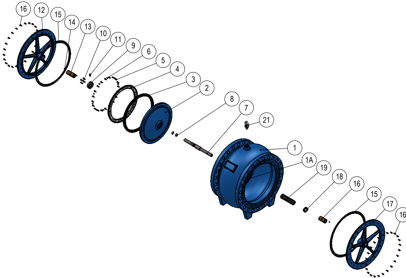
DN 125 - 1200 Parts List & Material Specification
